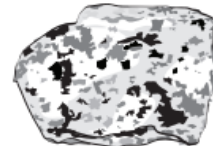
Igneous
