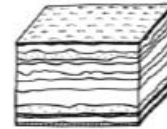
Sedimentary
