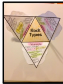
Types of Rocks Triangle
