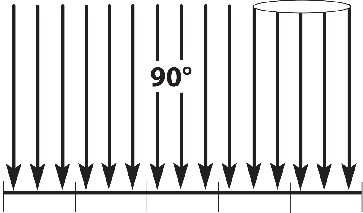
High (large) solar angle
