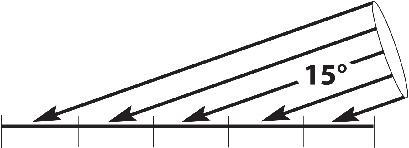
Low (small) solar angle
